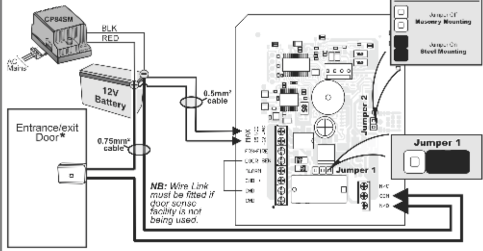
Fig 3. Wiring Diagram for Door Lock Type 1
