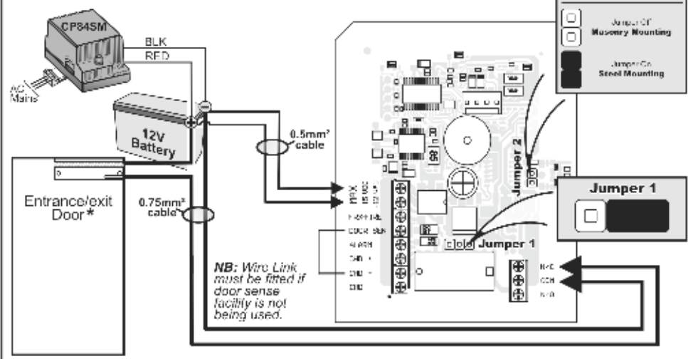
Fig 4. Wiring Diagram for Door Lock Type 2
